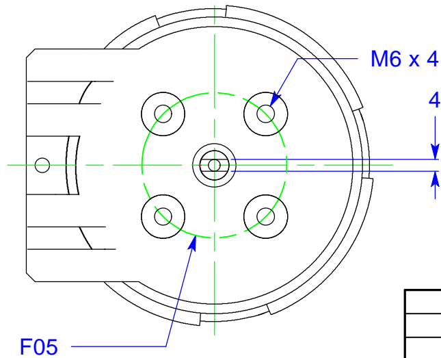
Type SLR Dimensional Drawing
